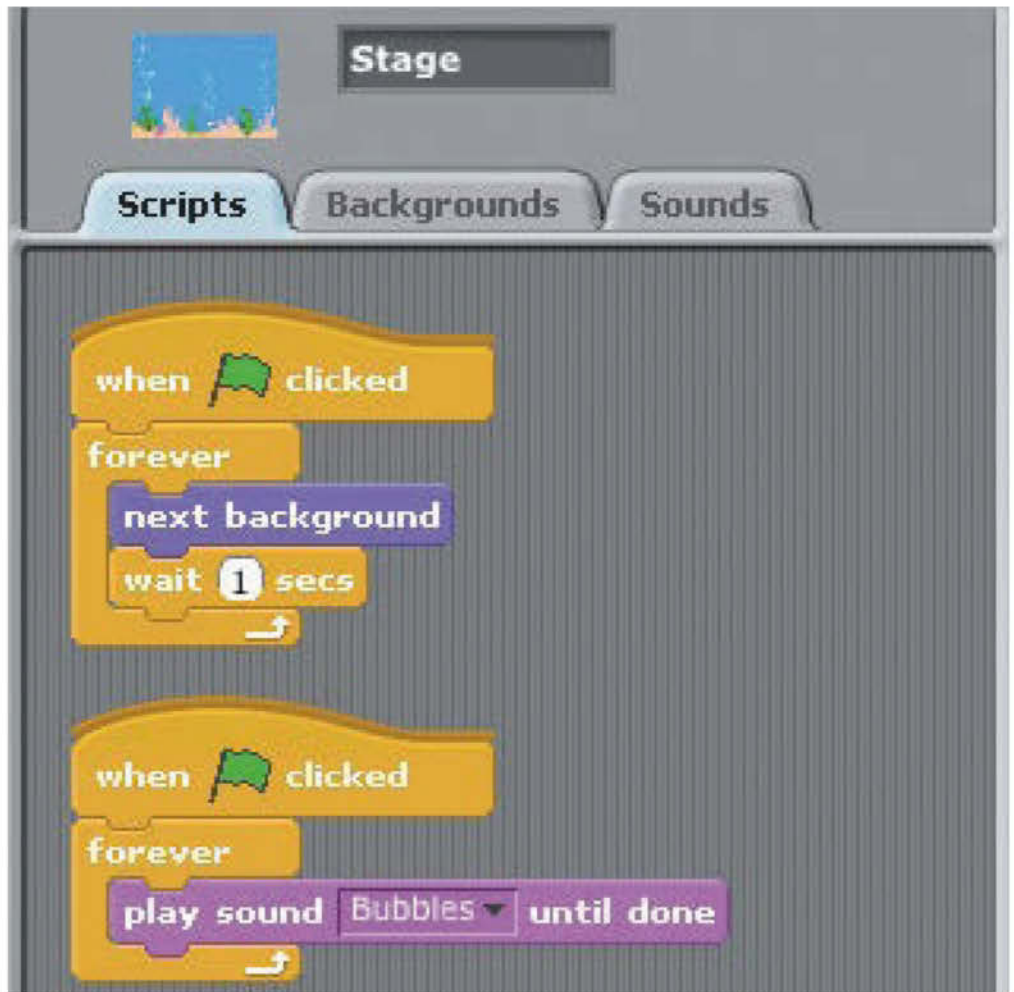
■ Fig 3: The Stage sprite's Script tab after adding the 'Bubbles' sound play block script
